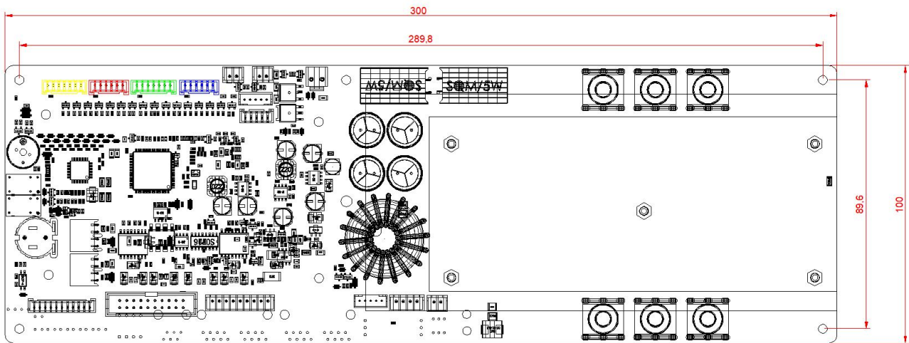
保护板尺寸图 (Dimensional figure of BMS)
